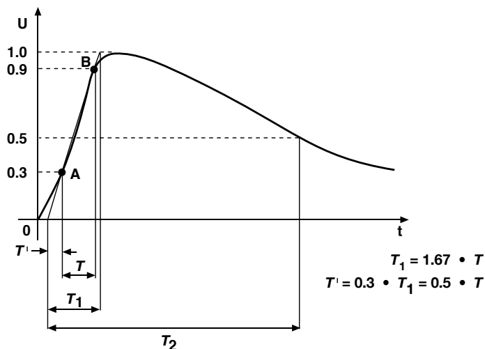
Figure 5. 1.2/50 \mu s or 10/700 \mu s single high voltage pulse.
